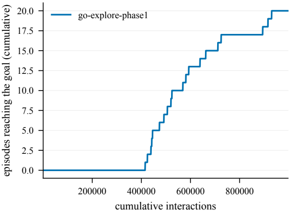
Goal reached -- EpicChase8-120@20
