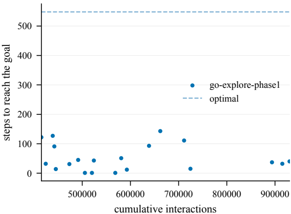
Steps to goal (train) -- EpicChase8-120@20
