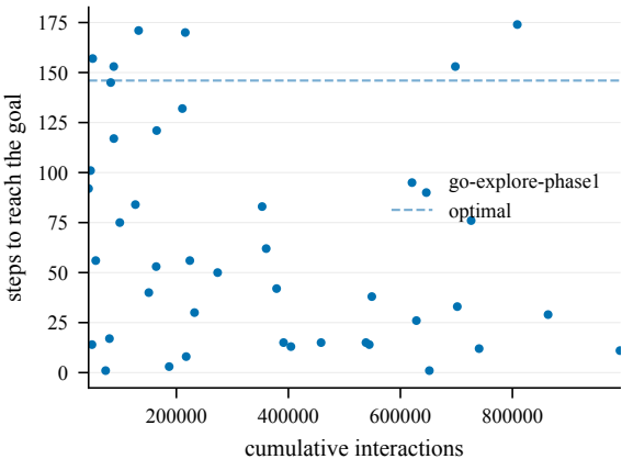
Steps to goal (train) -- EpicChase8-120@28
