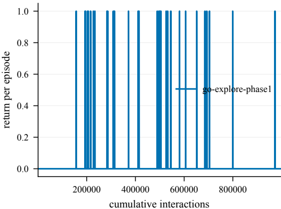
Return -- EpicChase8-120@29
