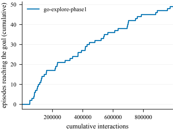
Goal reached -- EpicChase6-110
