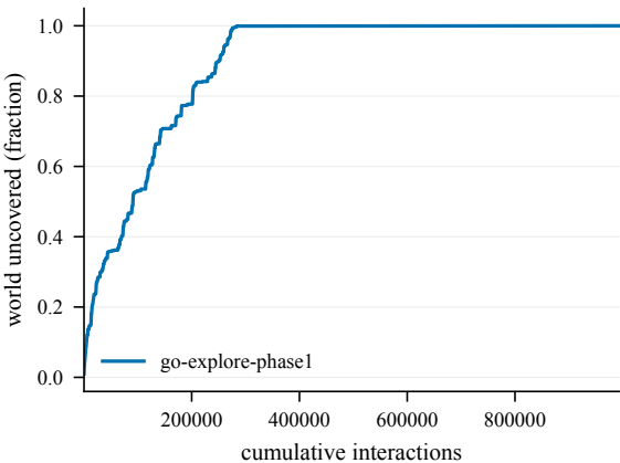
Cumulative coverage -- EpicChase1-60
