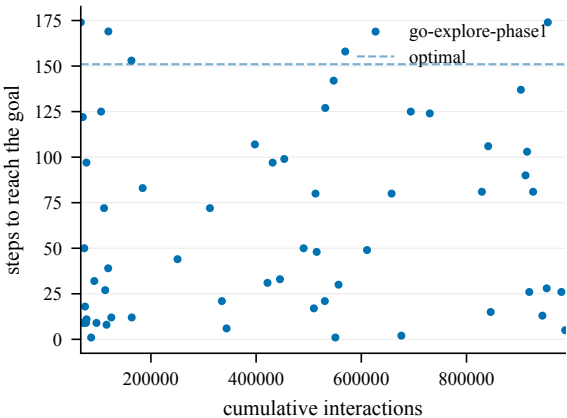
Steps to goal (train) -- EpicChase1-60
