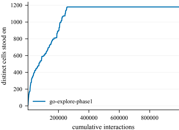
States discovered -- EpicChase1-60@1
