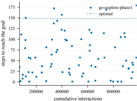
Steps to goal (train) -- EpicChase1-60@4
