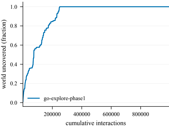
Cumulative coverage -- EpicChase1-60@5
