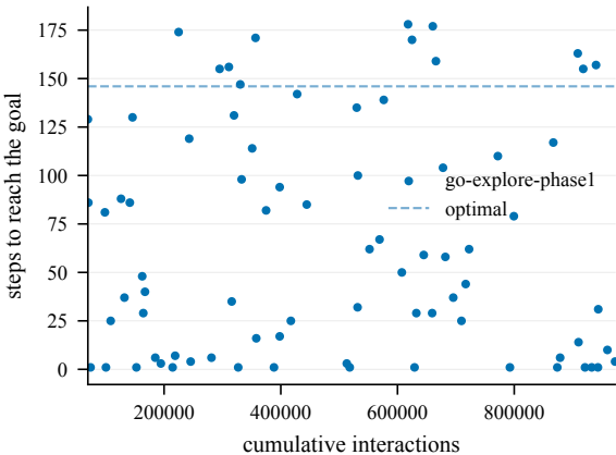
Steps to goal (train) -- EpicChase1-60@5
