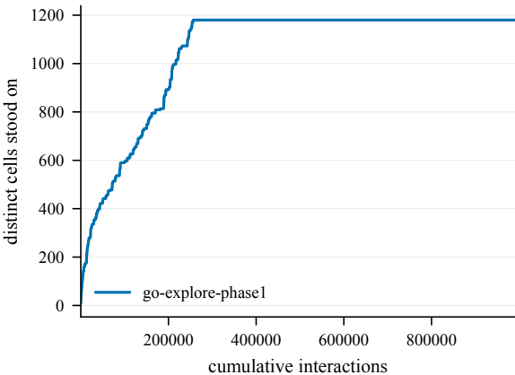
States discovered -- EpicChase1-60@6
