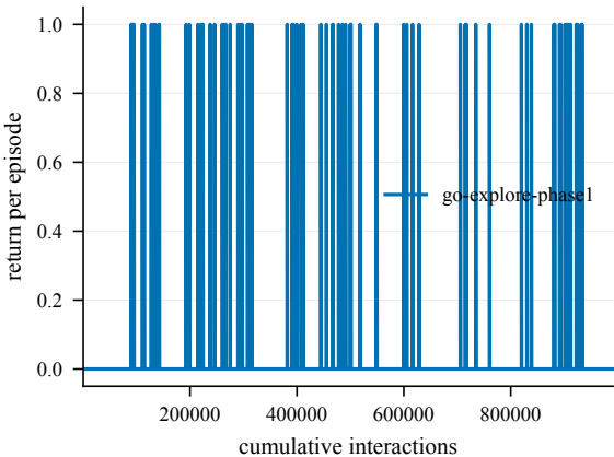
Return -- EpicChase1-60@8
