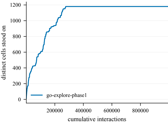
States discovered -- EpicChase1-60@8
