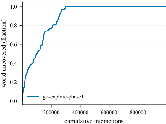
Cumulative coverage -- EpicChase1-60@9
