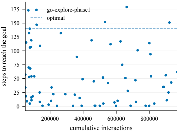
Steps to goal (train) -- EpicChase1-60@9
