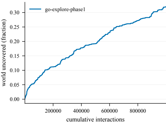
Cumulative coverage -- EpicChase12-150
