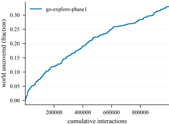
Cumulative coverage -- EpicChase12-150@1
