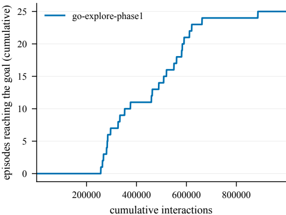
Goal reached -- EpicChase12-150@2
