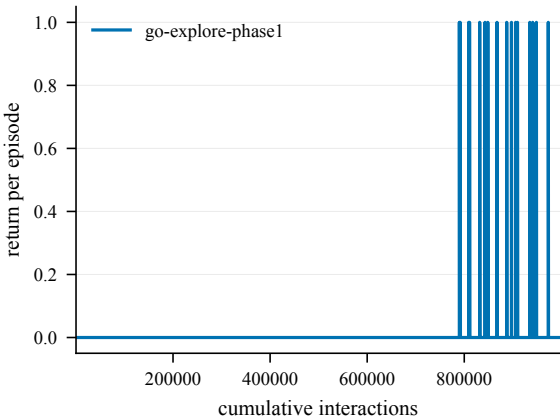
Return -- EpicChase12-150@3
