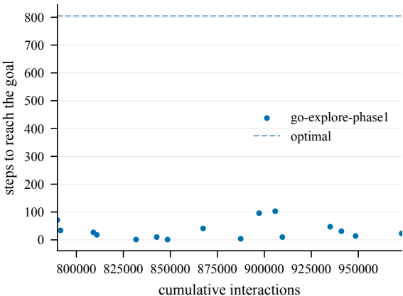
Steps to goal (train) -- EpicChase12-150@3
