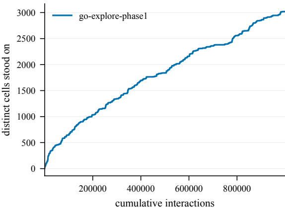
States discovered -- EpicChase12-150@6
