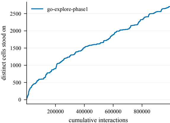
States discovered -- EpicChase12-150@7
