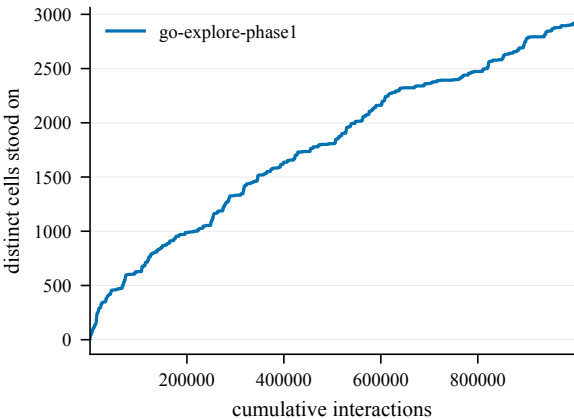
States discovered -- EpicChase12-150@8
