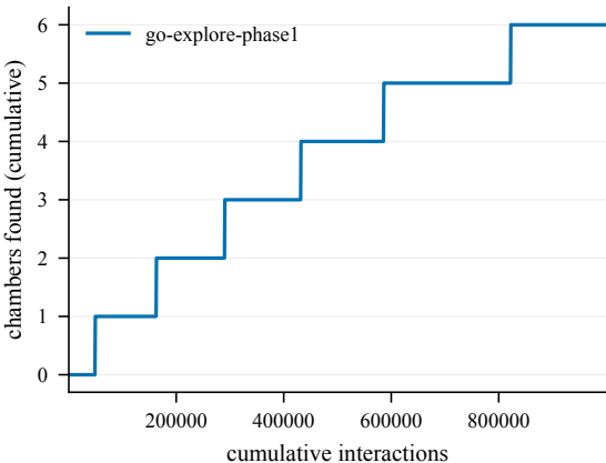
Chambers -- EpicChase12-150@9
