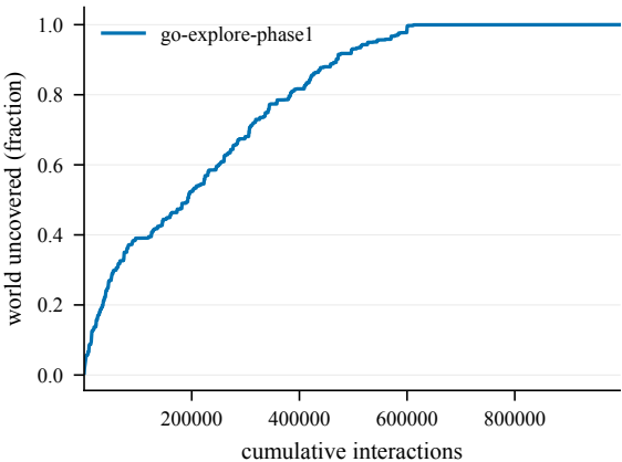
Cumulative coverage -- EpicChase2-70@3
