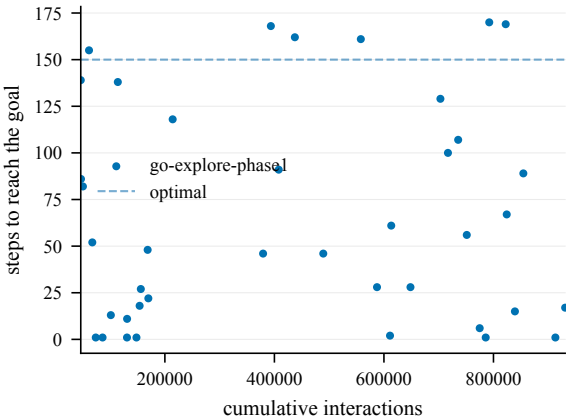
Steps to goal (train) -- EpicChase2-70@3
