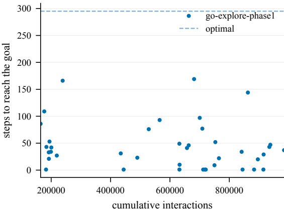
Steps to goal (train) -- EpicChase2-70@4
