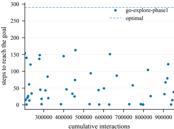
Steps to goal (train) -- EpicChase2-70@5
