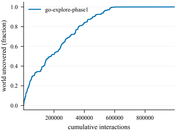
Cumulative coverage -- EpicChase2-70@6
