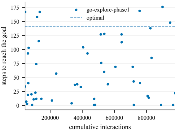
Steps to goal (train) -- EpicChase2-70@6
