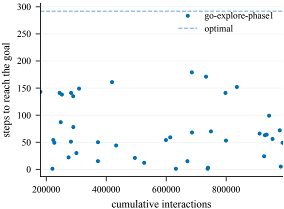
Steps to goal (train) -- EpicChase2-70@7
