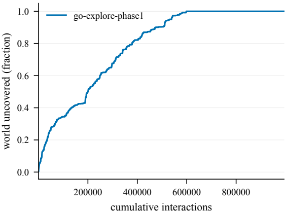
Cumulative coverage -- EpicChase2-70@9
