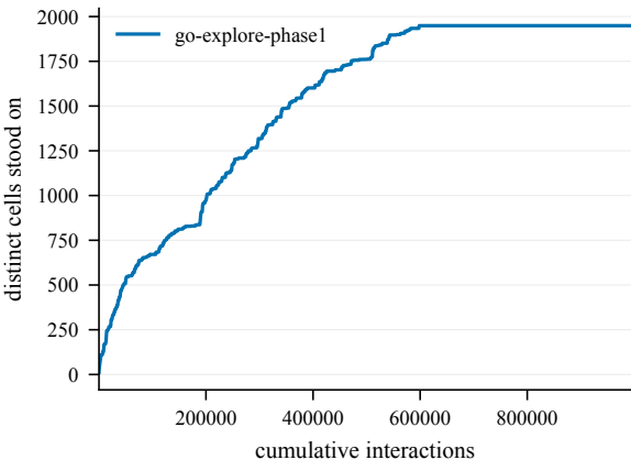
States discovered -- EpicChase2-70@9
