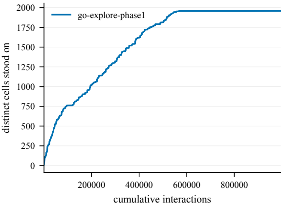
States discovered -- EpicChase3-70@3
