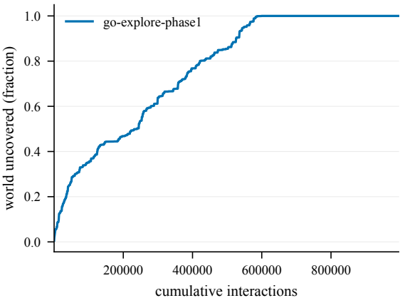
Cumulative coverage -- EpicChase3-70@5
