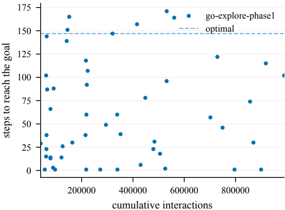
Steps to goal (train) -- EpicChase3-70@8
