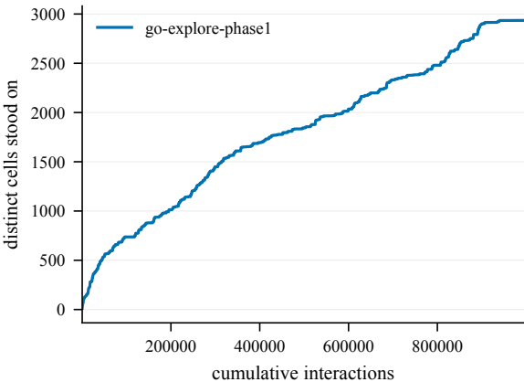
States discovered -- EpicChase4-90@1
