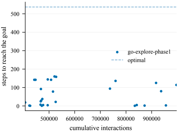
Steps to goal (train) -- EpicChase4-90@2
