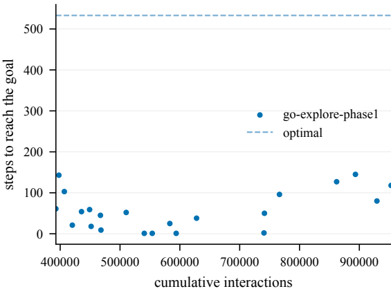
Steps to goal (train) -- EpicChase4-90@3
