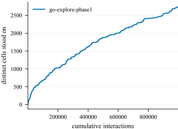
States discovered -- EpicChase4-90@4
