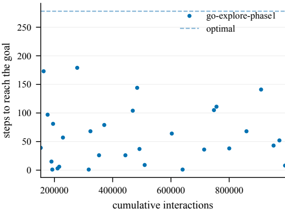
Steps to goal (train) -- EpicChase4-90@6
