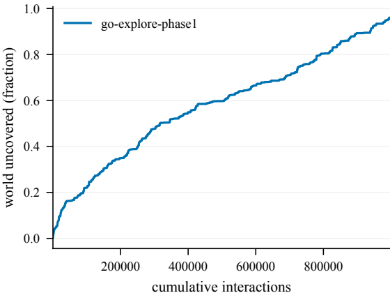
Cumulative coverage -- EpicChase4-90@7
