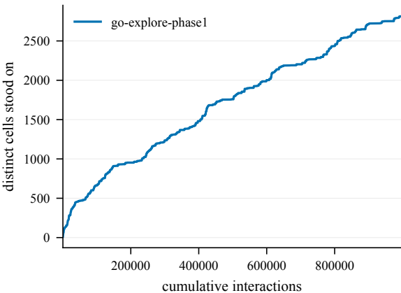
States discovered -- EpicChase4-90@8
