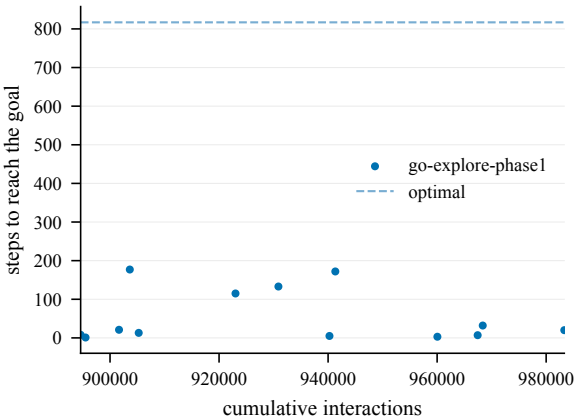
Steps to goal (train) -- EpicChase6-110@1
