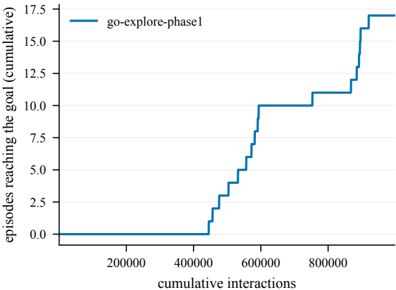
Goal reached -- EpicChase6-110@3
