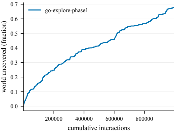
Cumulative coverage -- EpicChase6-110@5
