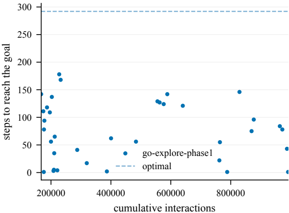
Steps to goal (train) -- EpicChase6-110@7
