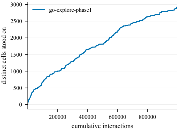
States discovered -- EpicChase6-110@8
