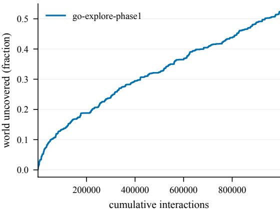
Cumulative coverage -- EpicChase8-120@1
